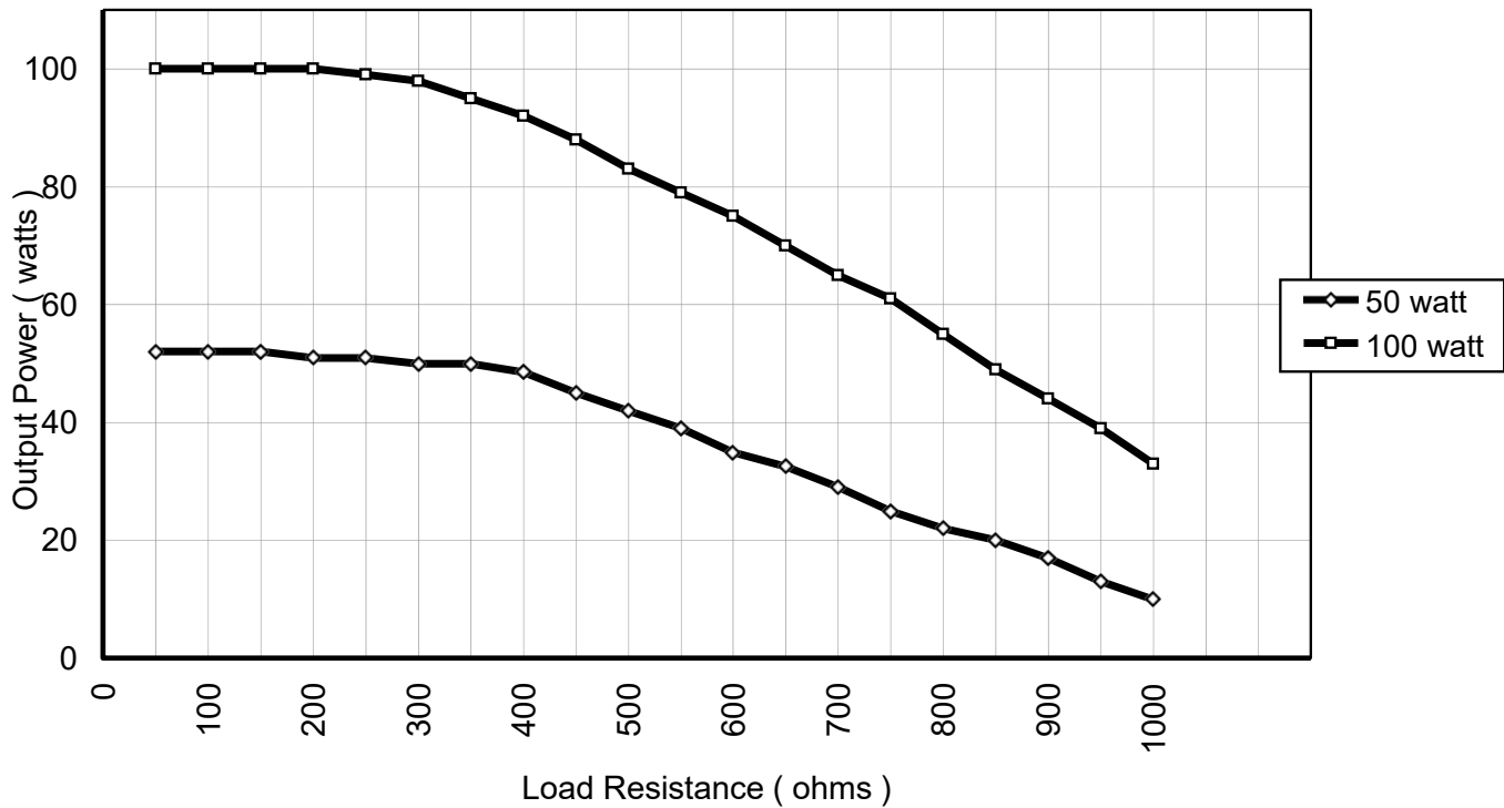
Bipolar mode - Force
