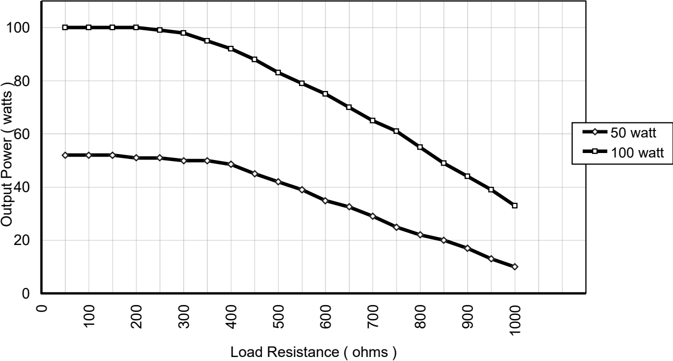
Bipolar mode - Bicut/Macro
