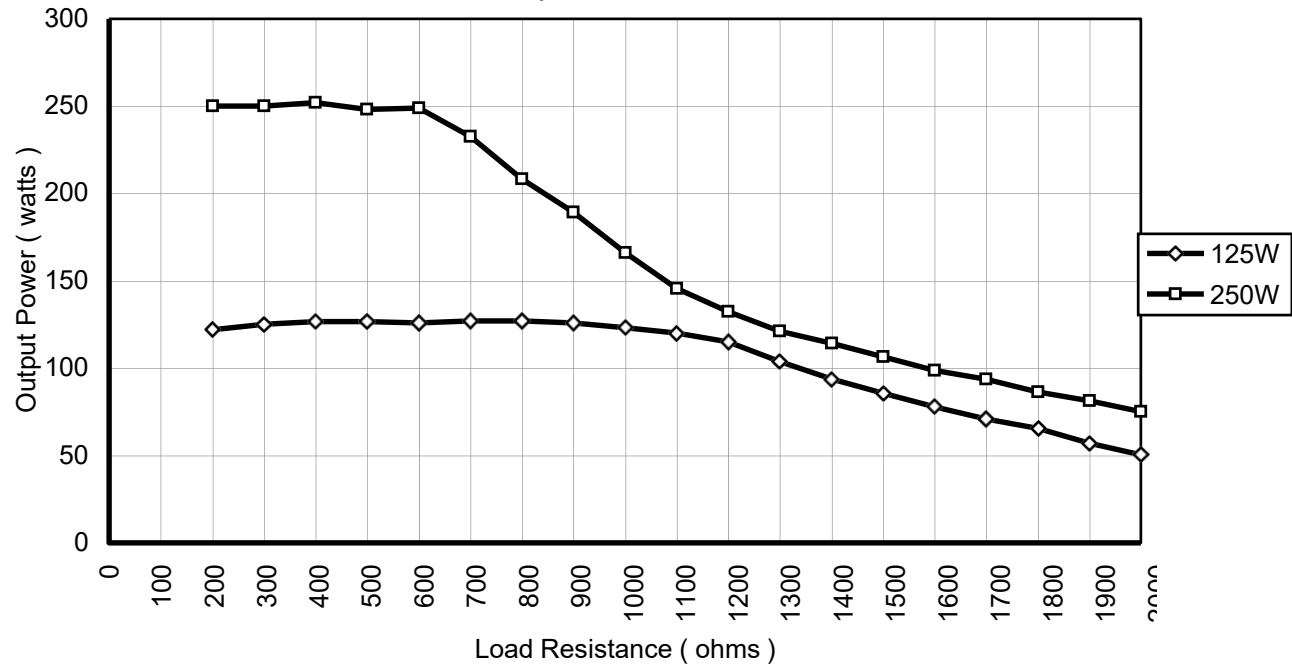
Monopolar BlendCut Mode
